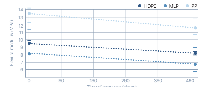
Figure 87 Flexural modulus over time of exposure
