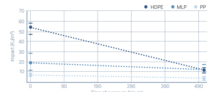
Figure 88 Charpy impact strength over time of exposure
